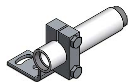
Clamping collar with angle PS 11/K-35 AF 2
